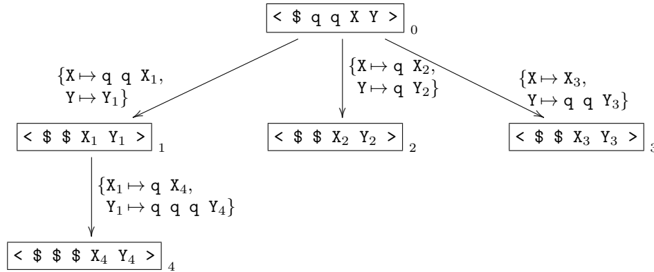
Figure 12.1: Folding variant narrowing tree for the term \langle \$ q q X Y \rangle .
