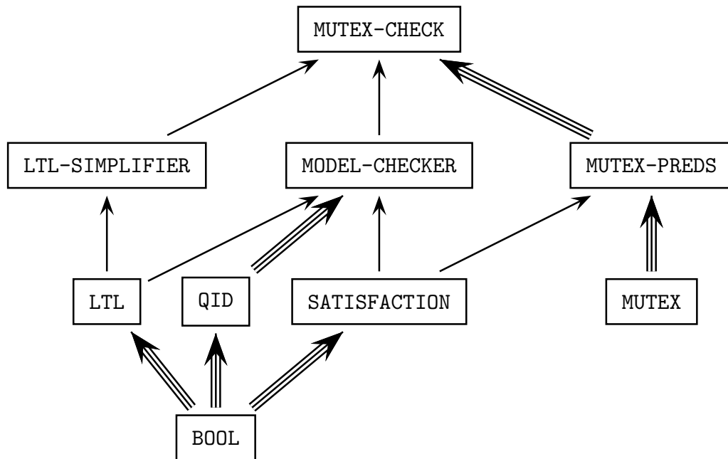
Figure 10.1: Importation graph of model-checking modules
