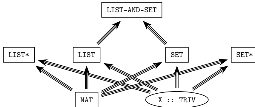
Figure 8.2: Importation graph of parameterized list and set modules
