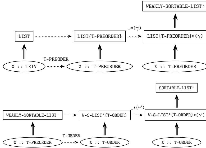
Figure 8.5: Another version of sortable lists
