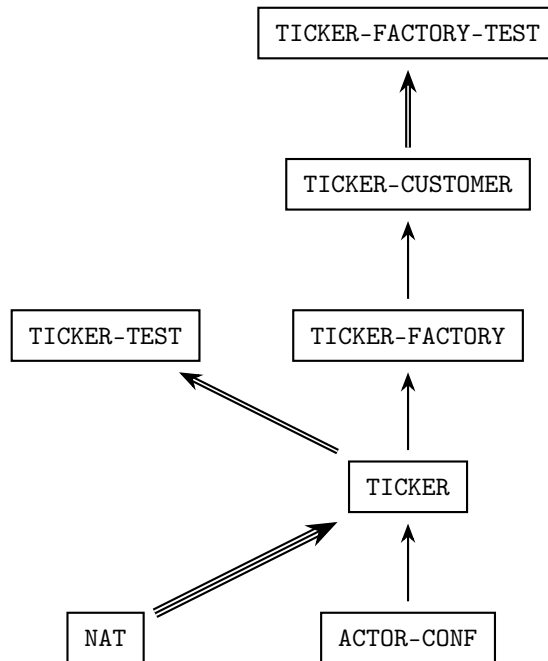
Figure 6.2: Importation graph of ticker modules
