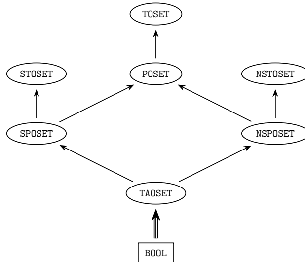
Figure 7.1: Hierarchy of order theories
