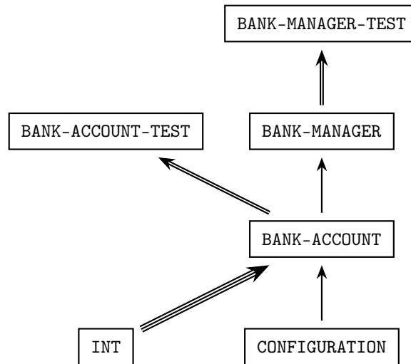
Figure 6.1: Importation graph of bank modules
