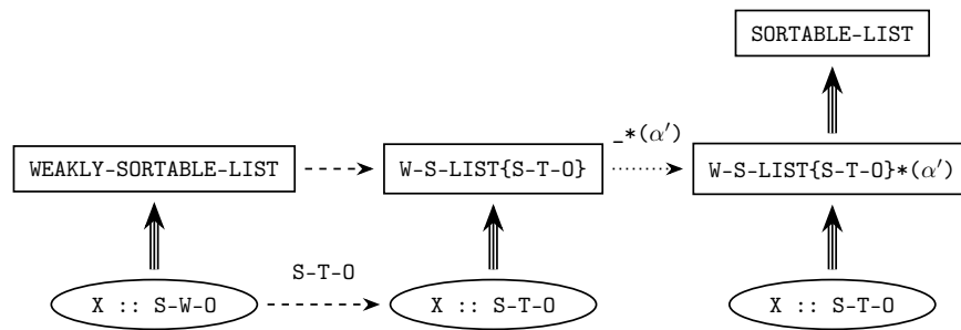
Figure 8.4: From weakly sortable lists to sortable lists
