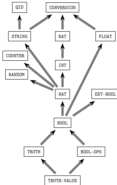
Figure 8.1: Importation (protecting) graph of predefined modules
