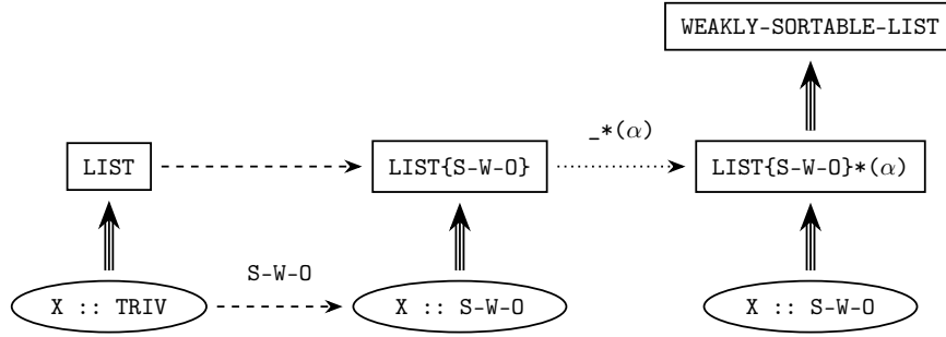
Figure 8.3: From lists to weakly sortable lists
