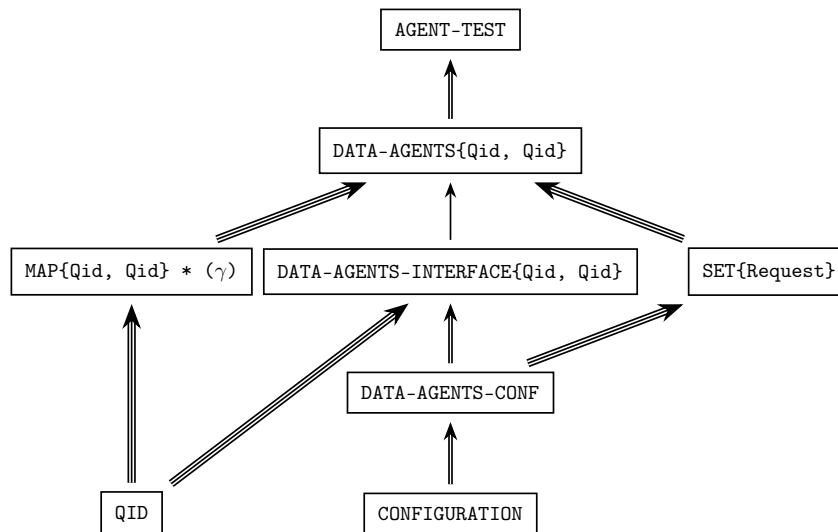
Figure 7.3: Importation graph of data-agents modules
